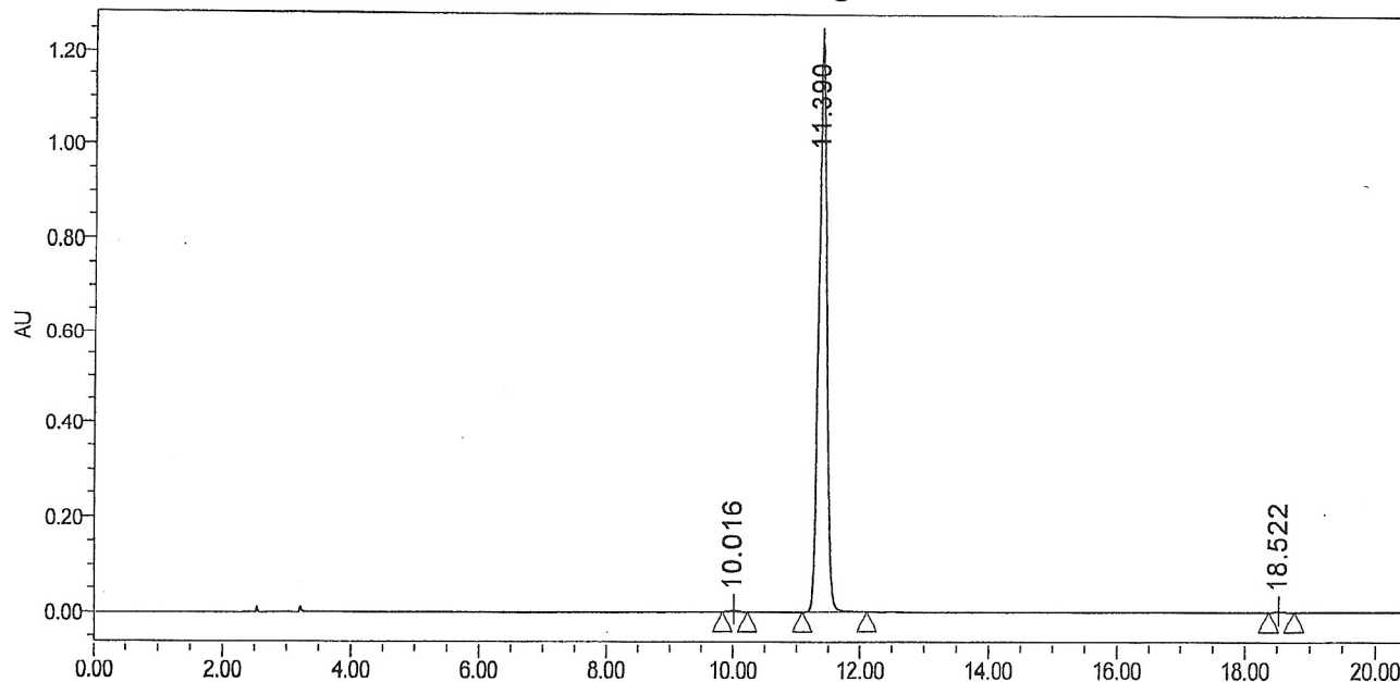
Auto-Scaled Chromatogram
